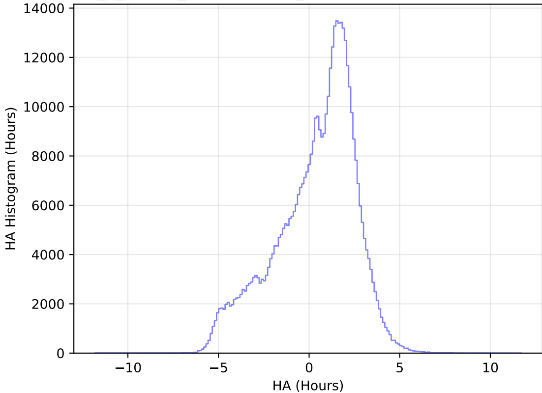
internal_u_expt45_nscale1.5v3.4_10yrs All sky r band: HA Histogram
