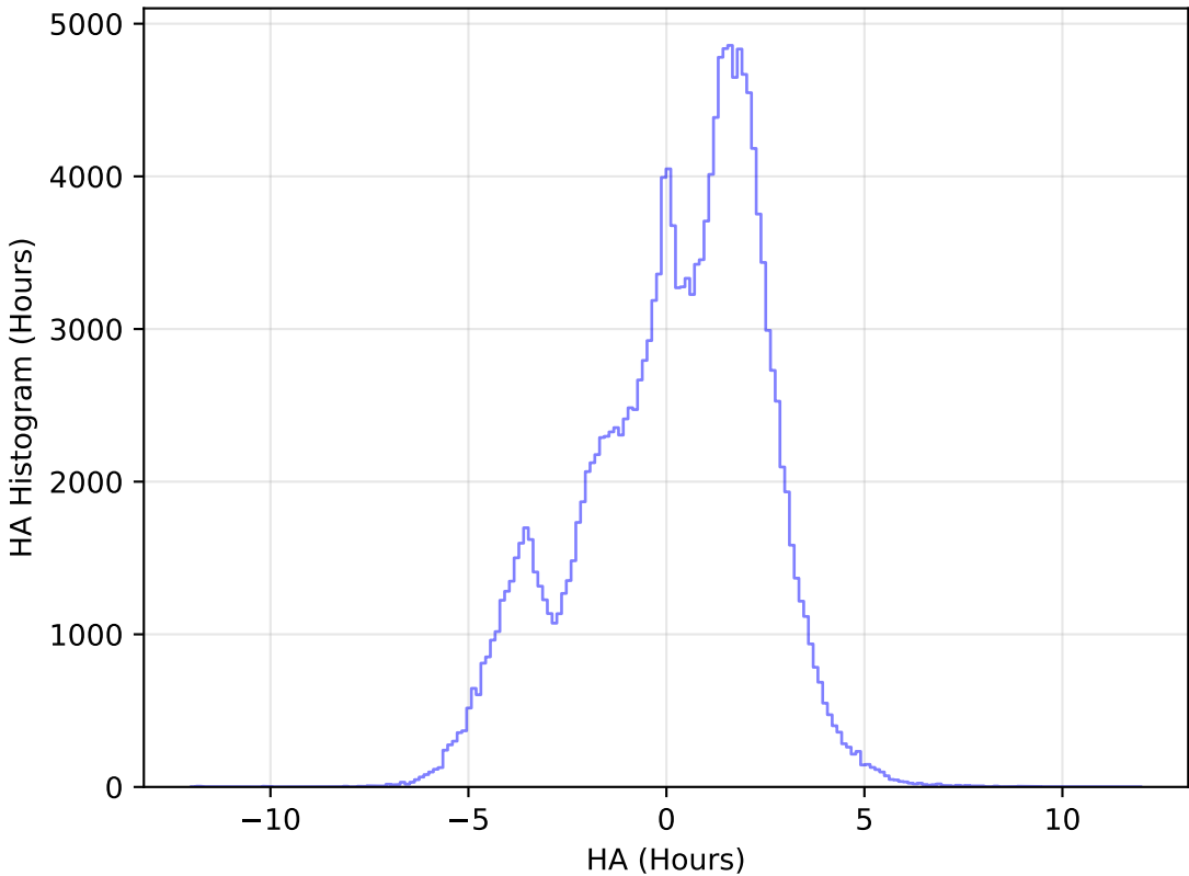
internal_u_expt45_nscale1.5v3.4_10yrs All sky g band: HA Histogram
