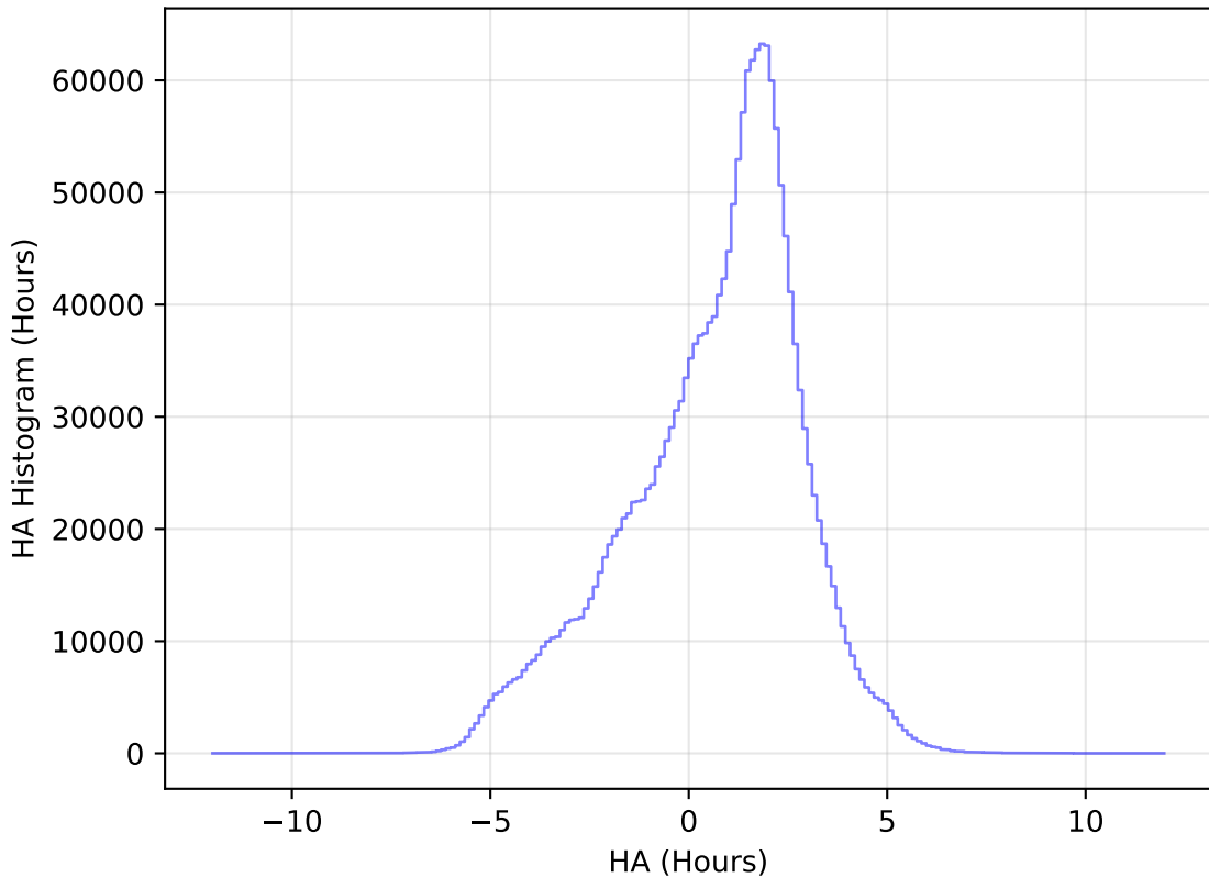
internal_u_expt45_nscale1.5v3.4_10yrs All sky all bands: HA Histogram
