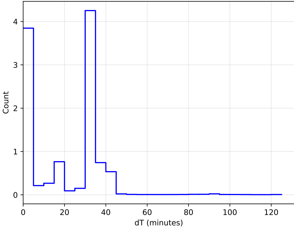
internal_u_expt45_nscale1.5v3.4_10yrs WFD: DeltaT Histogram
