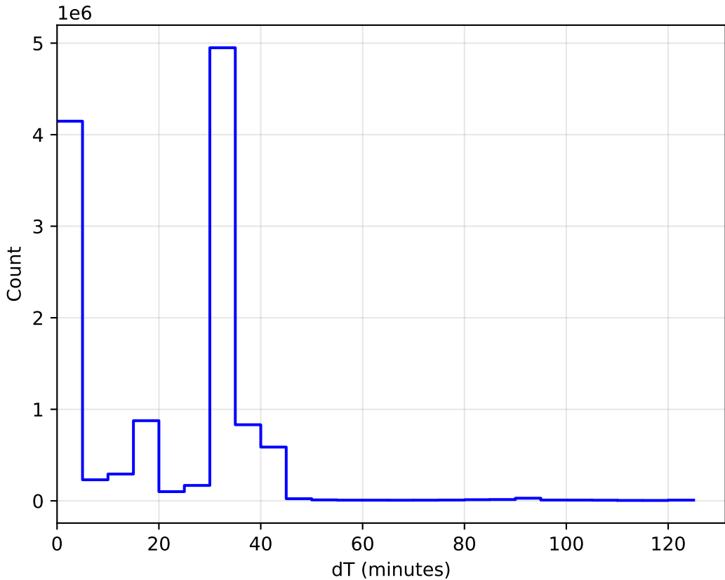
internal_u_expt45_nscale1.5v3.4_10yrs All sky: DeltaT Histogram
