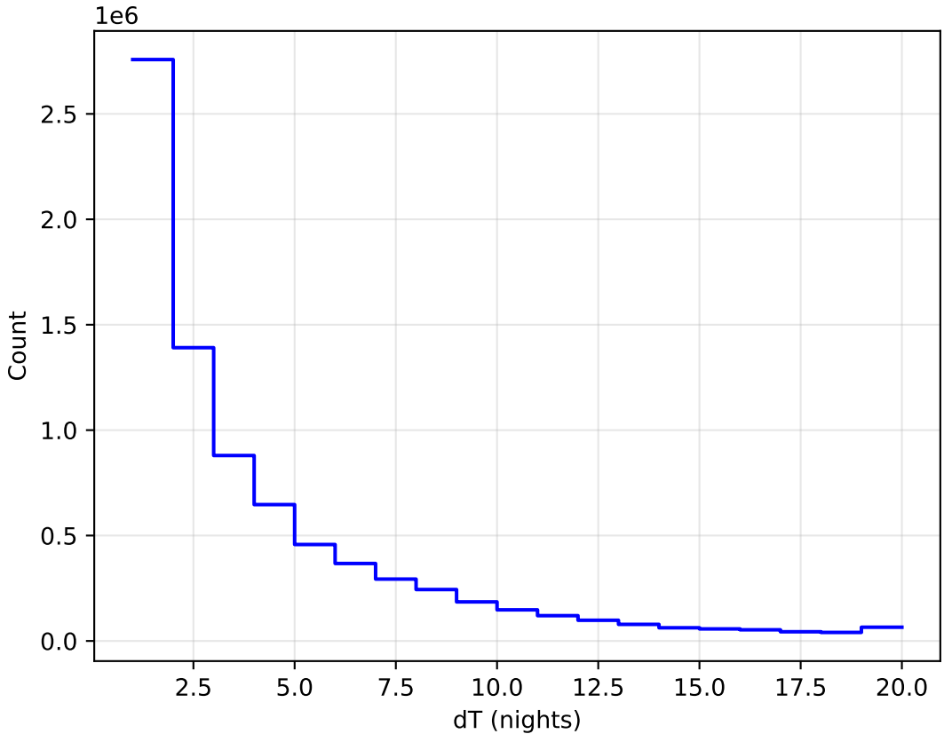
internal_u_expt45_nscale1.5v3.4_10yrs WFD all bands: DeltaNight Histogram
