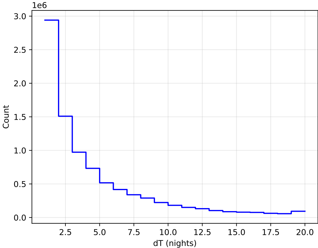
internal_u_expt45_nscale1.5v3.4_10yrs All sky all bands: DeltaNight Histogram
