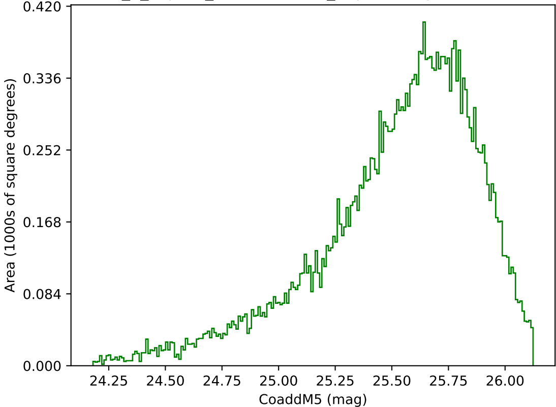
internal_u_expt45_nscale1.5v3.4_10yrs Yr 1 g band: CoaddM5
