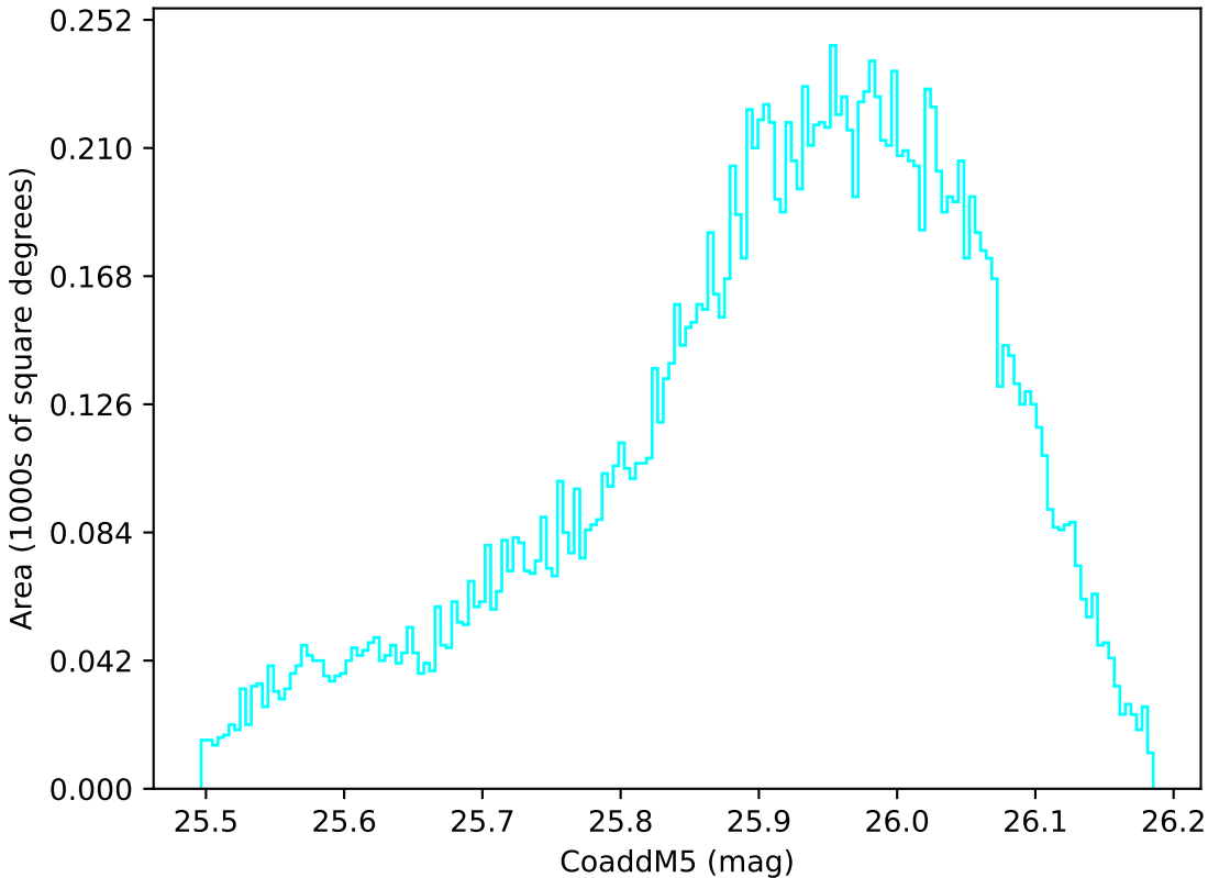
internal_u_expt45_nscale1.5v3.4_10yrs WFD u band: CoaddM5
