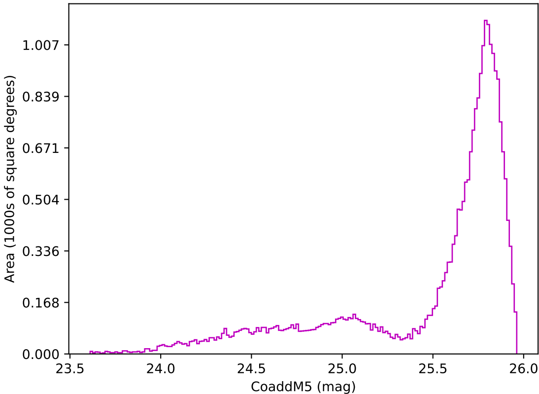
internal_u_expt45_nscale1.5v3.4_10yrs All sky z band: CoaddM5
