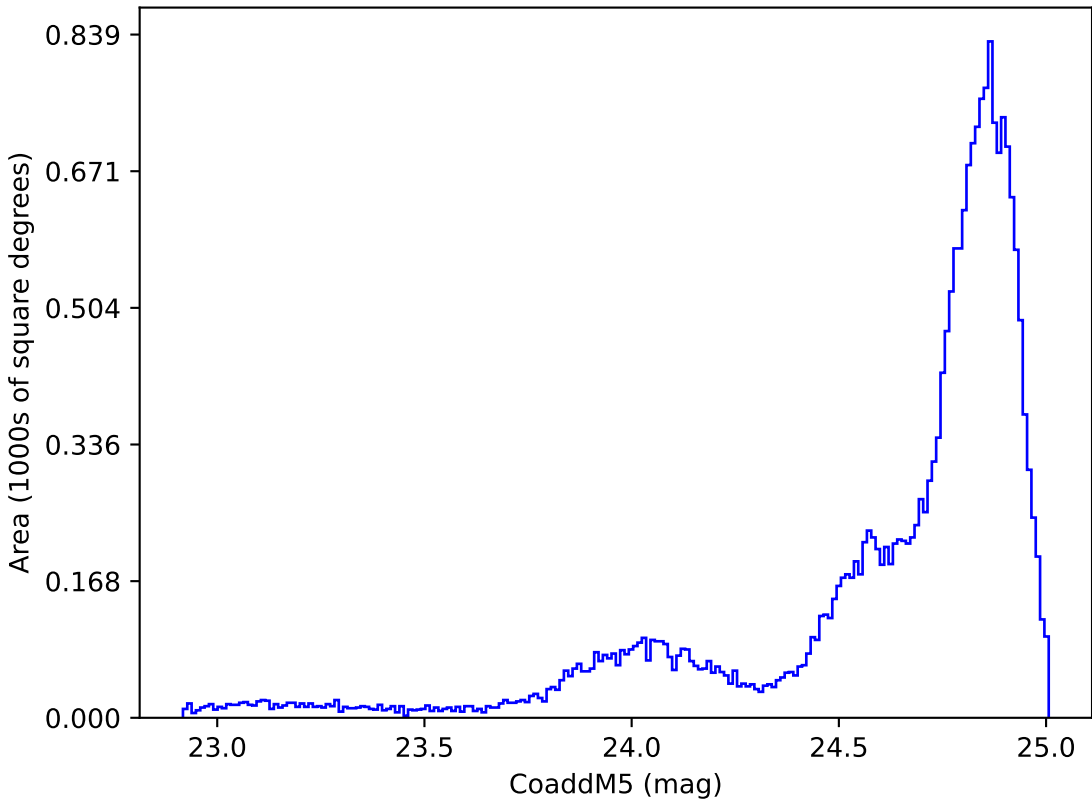
internal_u_expt45_nscale1.5v3.4_10yrs All sky y band: CoaddM5
