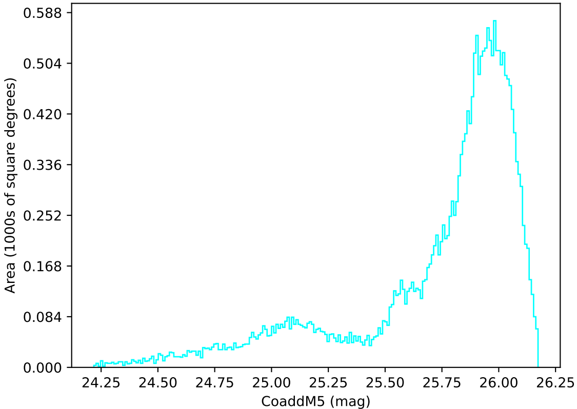
internal_u_expt45_nscale1.5v3.4_10yrs All sky u band: CoaddM5
