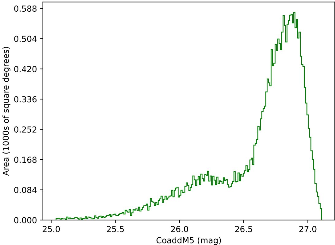
internal_u_expt45_nscale1.5v3.4_10yrs All sky g band: CoaddM5
