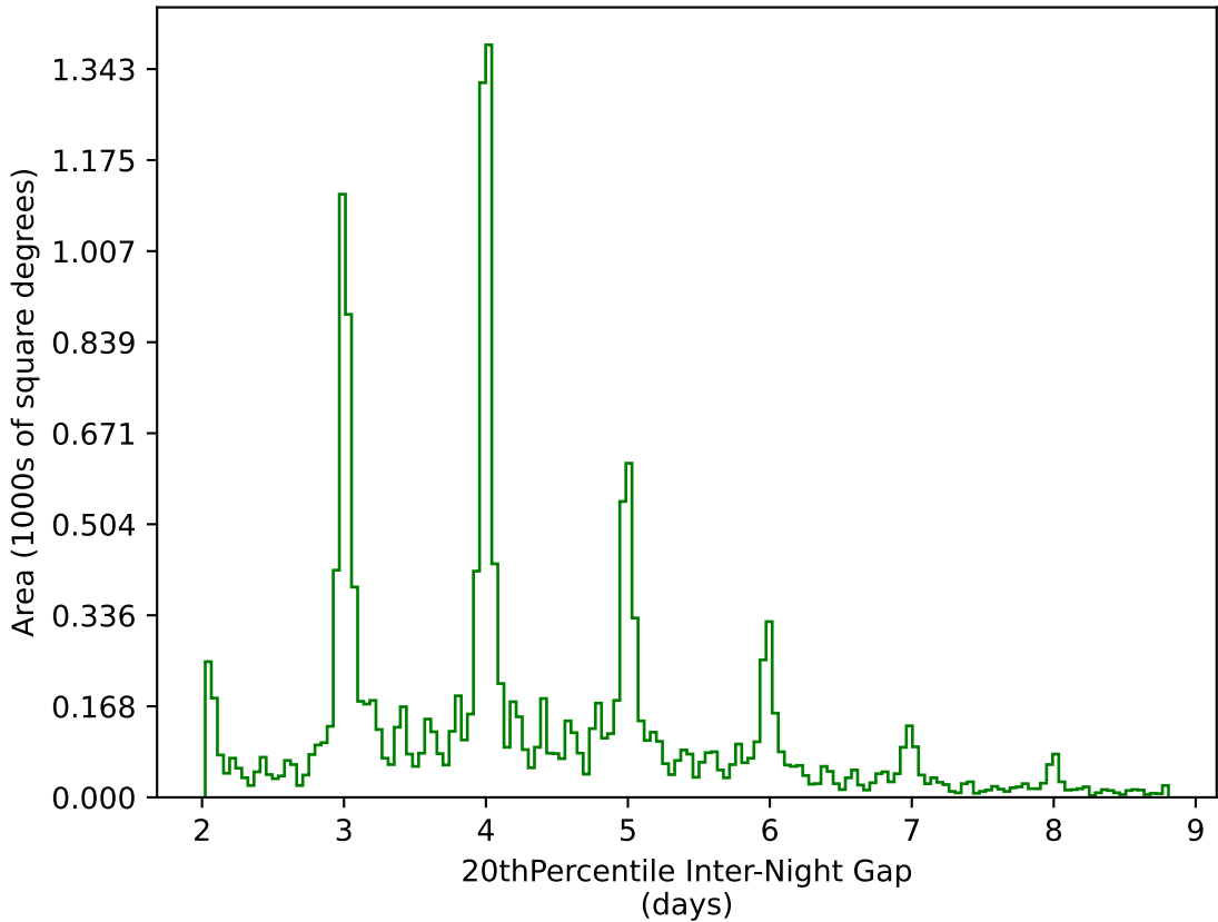
internal_u_expt45_nscale1.5v3.4_10yrs WFD g band: 20thPercentile Inter-Night Gap
