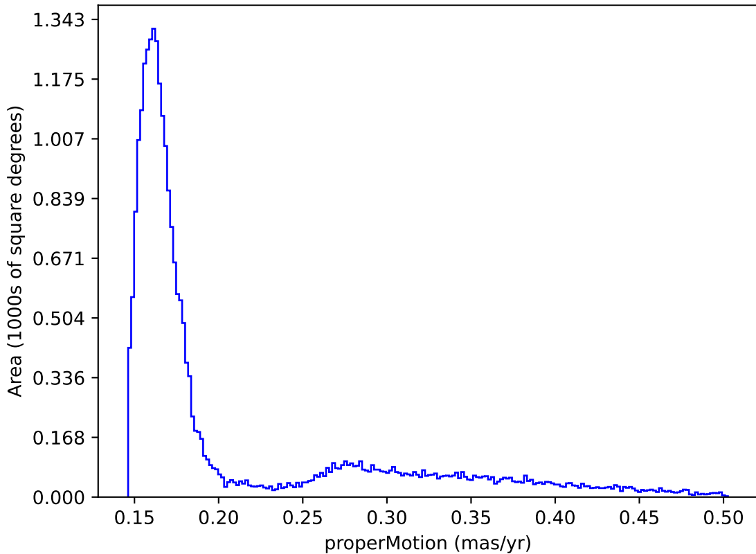
internal_u_expt45_nscale1.5v3.4_10yrs : properMotion
