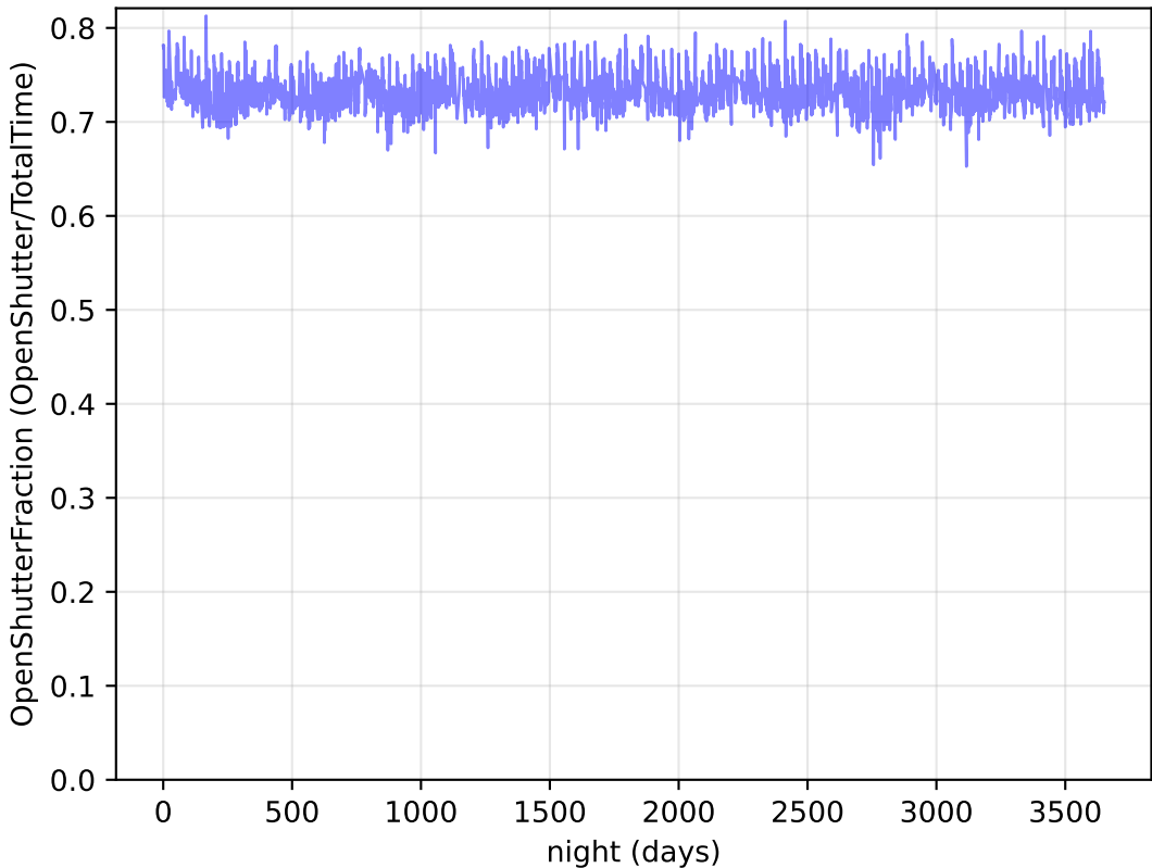
internal_u_expt45_nscale1.5v3.4_10yrs : OpenShutterFraction
