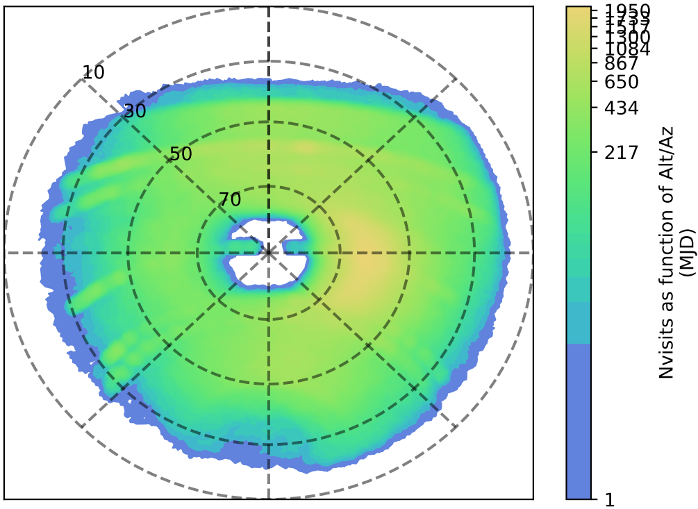
internal_u_expt45_nscale1.5v3.4_10yrs y: Nvisits as function of Alt/Az
