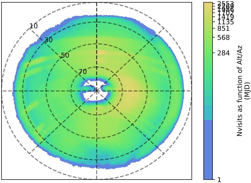
internal_u_expt45_nscale1.5v3.4_10yrs i: Nvisits as function of Alt/Az
