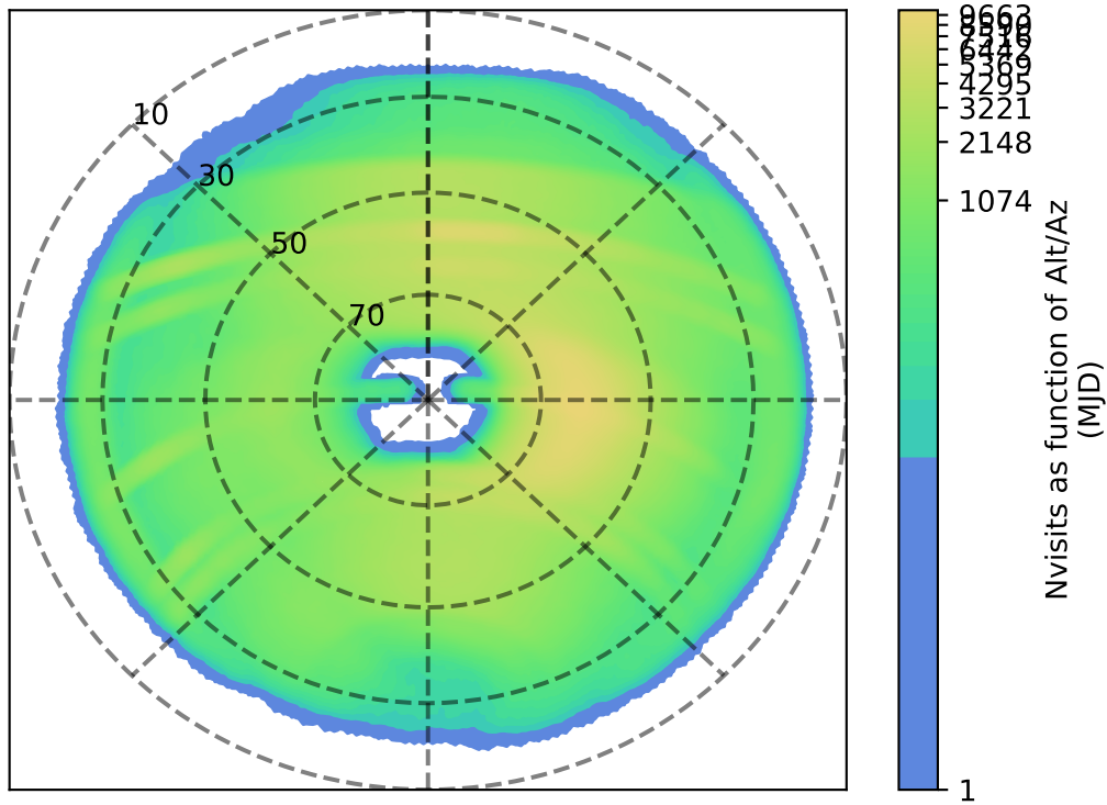
internal_u_expt45_nscale1.5v3.4_10yrs : Nvisits as function of Alt/Az
