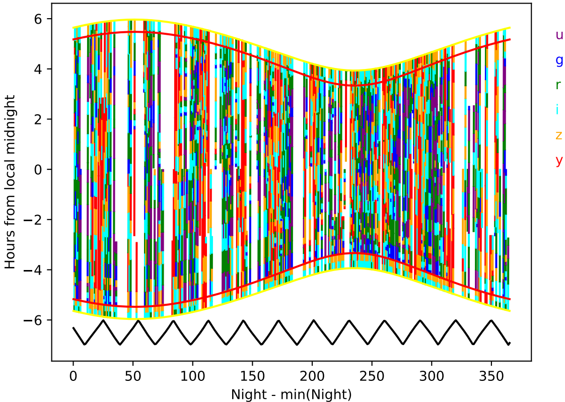
internal_u_expt45_nscale1.5v3.4_10yrs year 7-8: Hourglass
