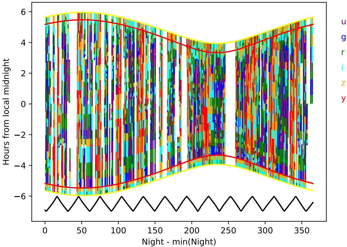
internal_u_expt45_nscale1.5v3.4_10yrs year 5-6: Hourglass
