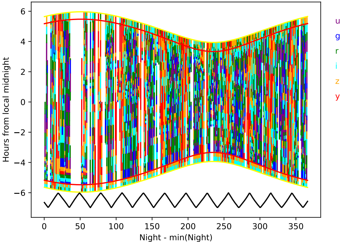
internal_u_expt45_nscale1.5v3.4_10yrs year 2-3: Hourglass
