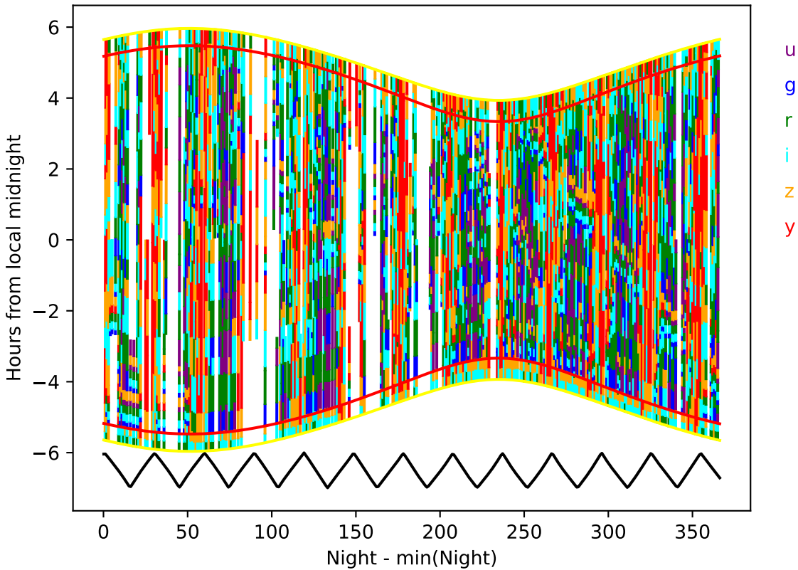
internal_u_expt45_nscale1.5v3.4_10yrs year 1-2: Hourglass
