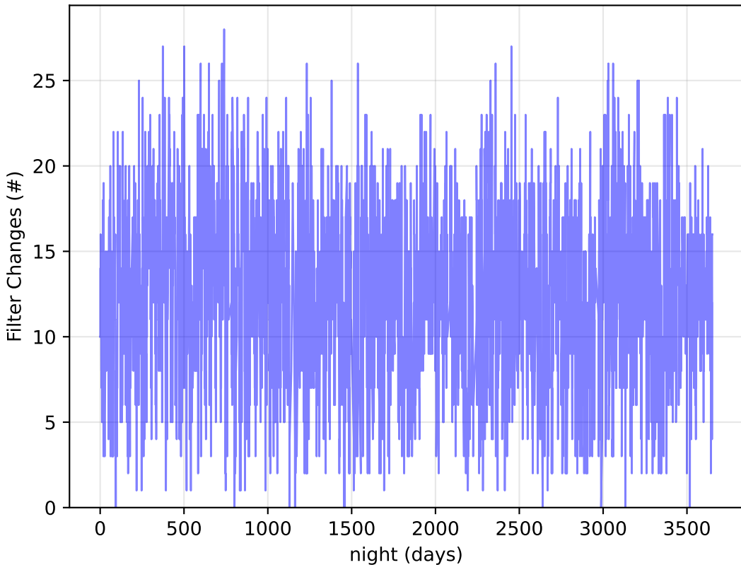
internal_u_expt45_nscale1.5v3.4_10yrs : Filter Changes
