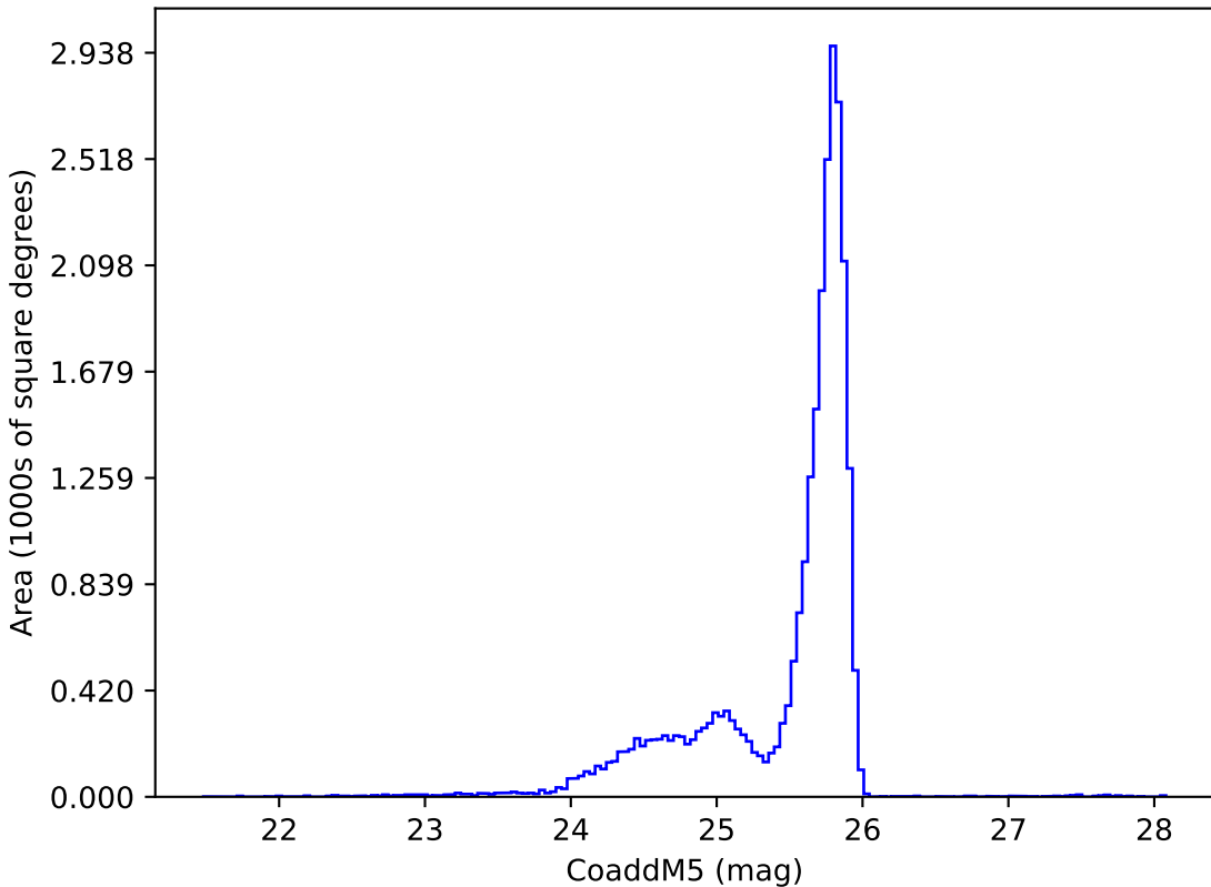
internal_u_expt45_nscale1.5v3.4_10yrs z: CoaddM5
