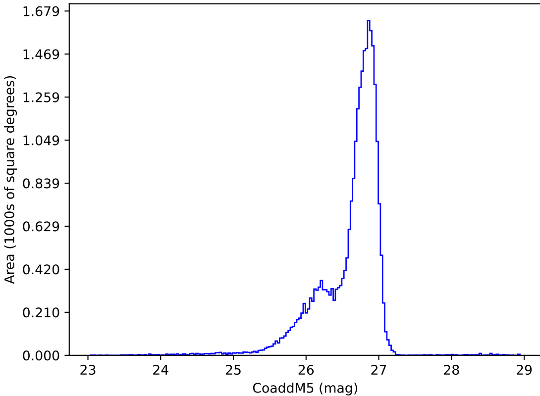
internal_u_expt45_nscale1.5v3.4_10yrs g: CoaddM5
