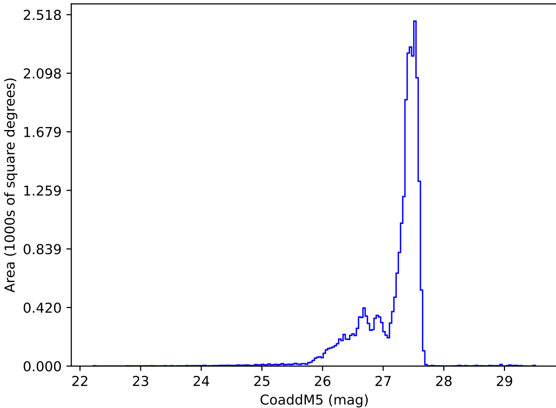
internal_u_expt45_nscale1.5v3.4_10yrs : CoaddM5
