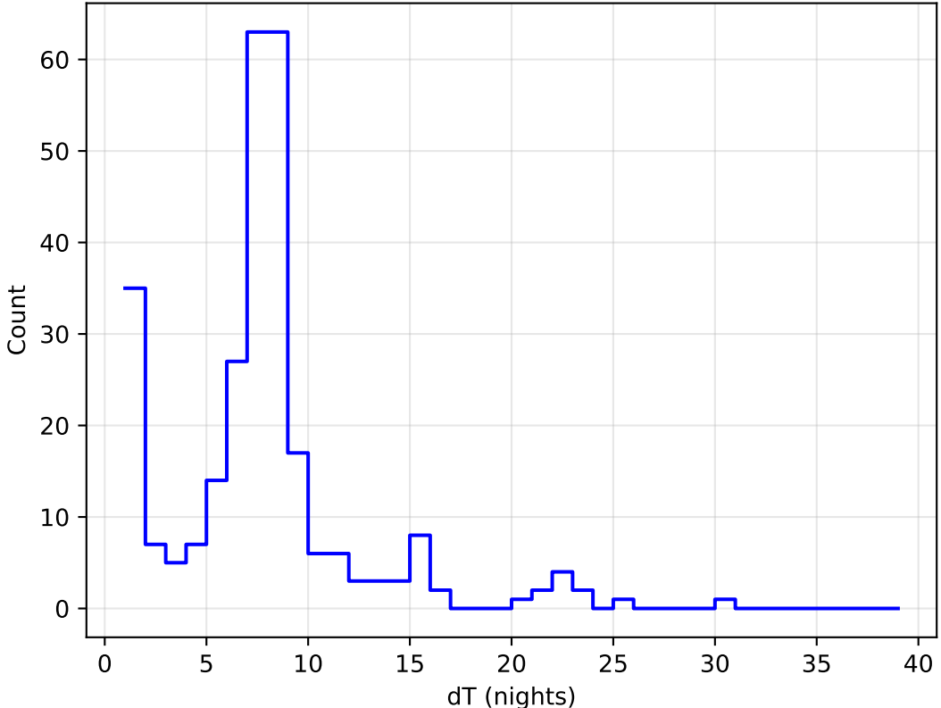
internal_u_expt45_nscale1.5v3.4_10yrs all bands: DD:ECDFS Delta Nights Histogram
