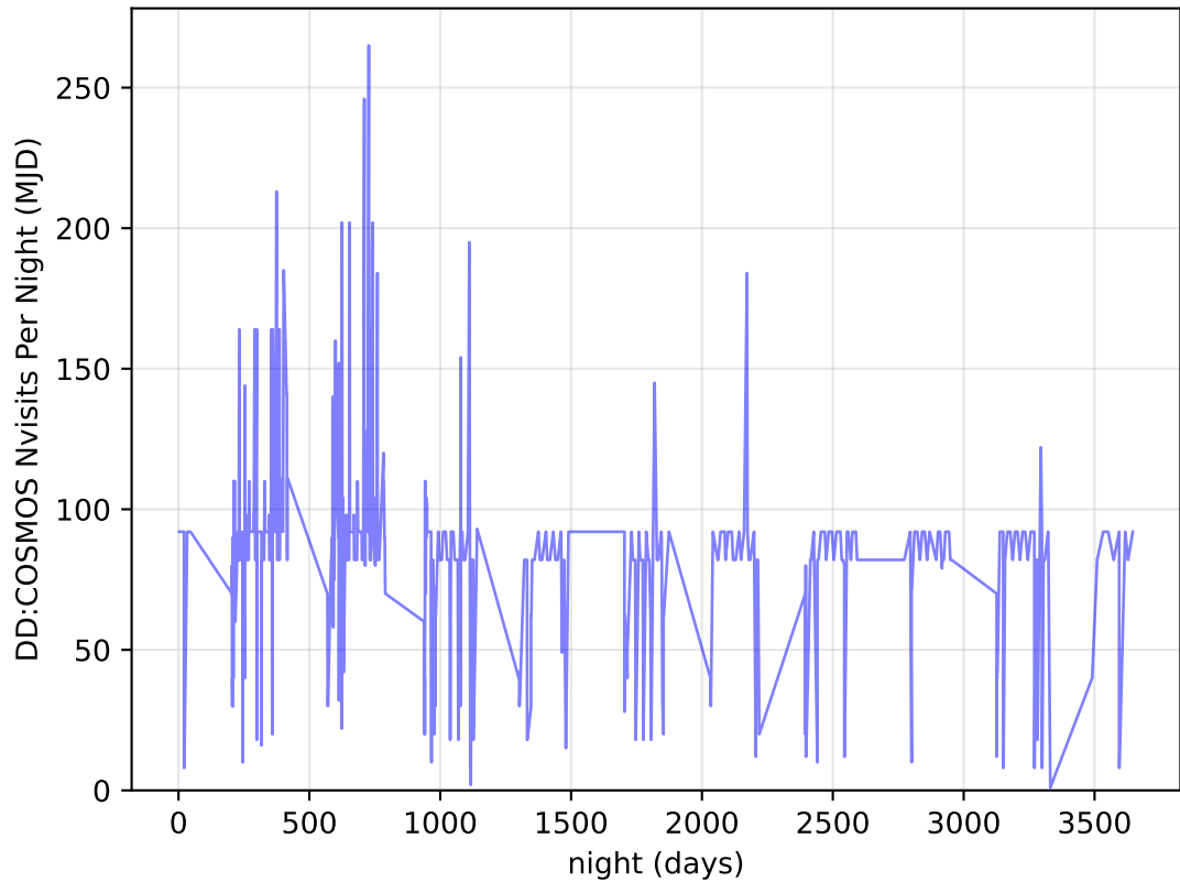
internal_u_expt45_nscale1.5v3.4_10yrs all bands: DD: COSMOS Nvisits Per Night
