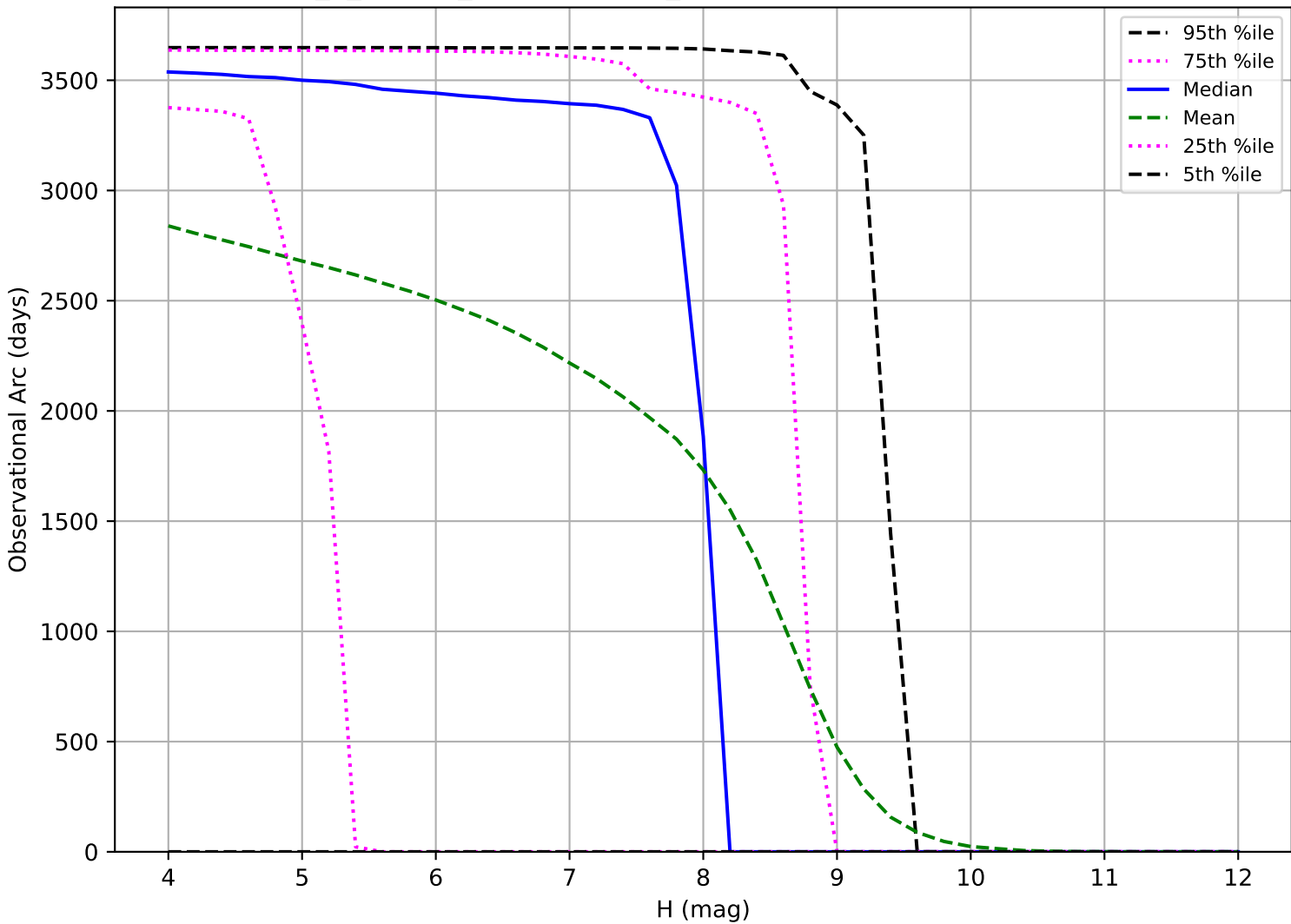
internal_u_expt45_nscale1.2v3.4_10yrs: Observational Arc Length TNO
