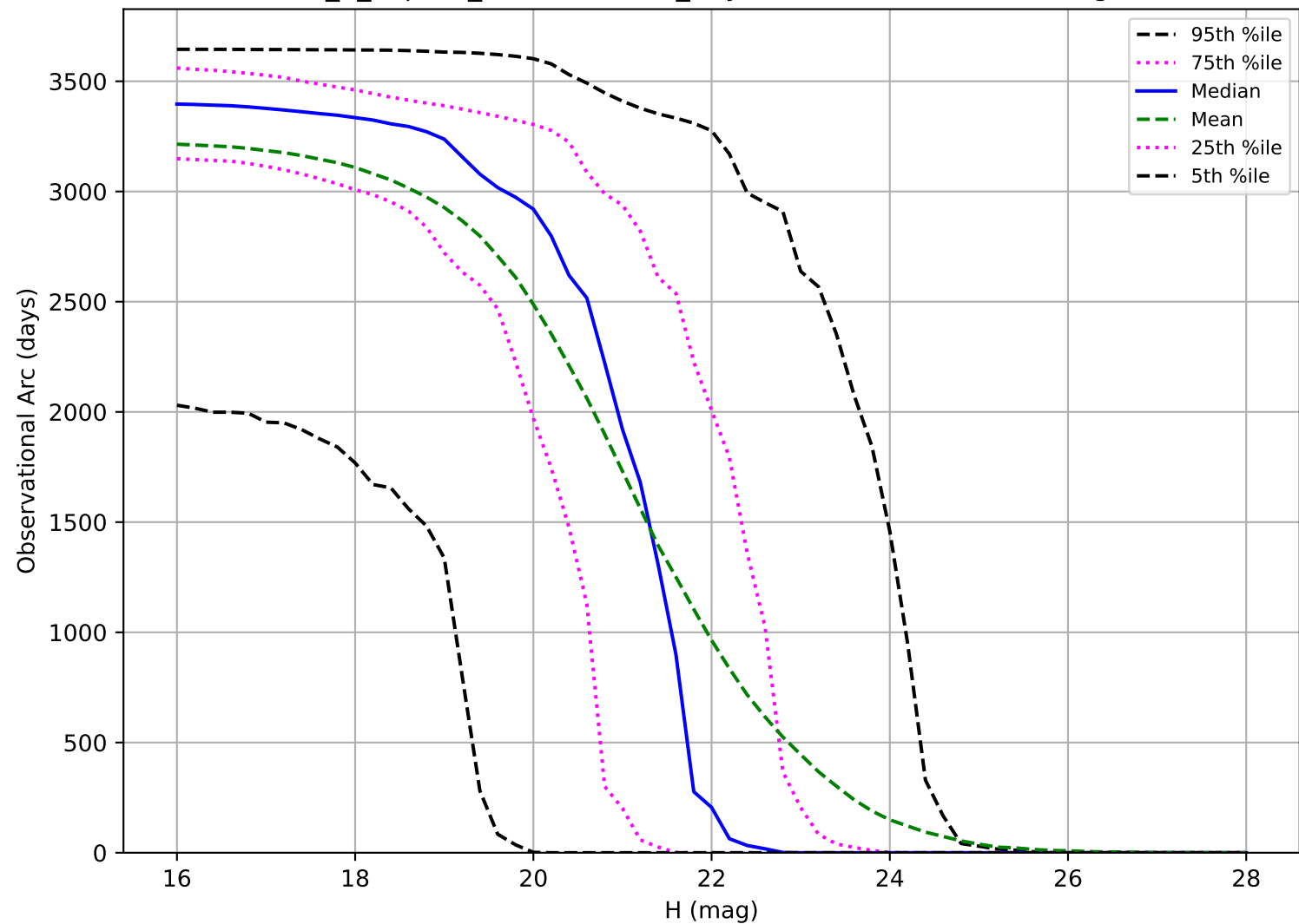
internal_u_expt45_nscale1.2v3.4_10yrs: Observational Arc Length PHA
