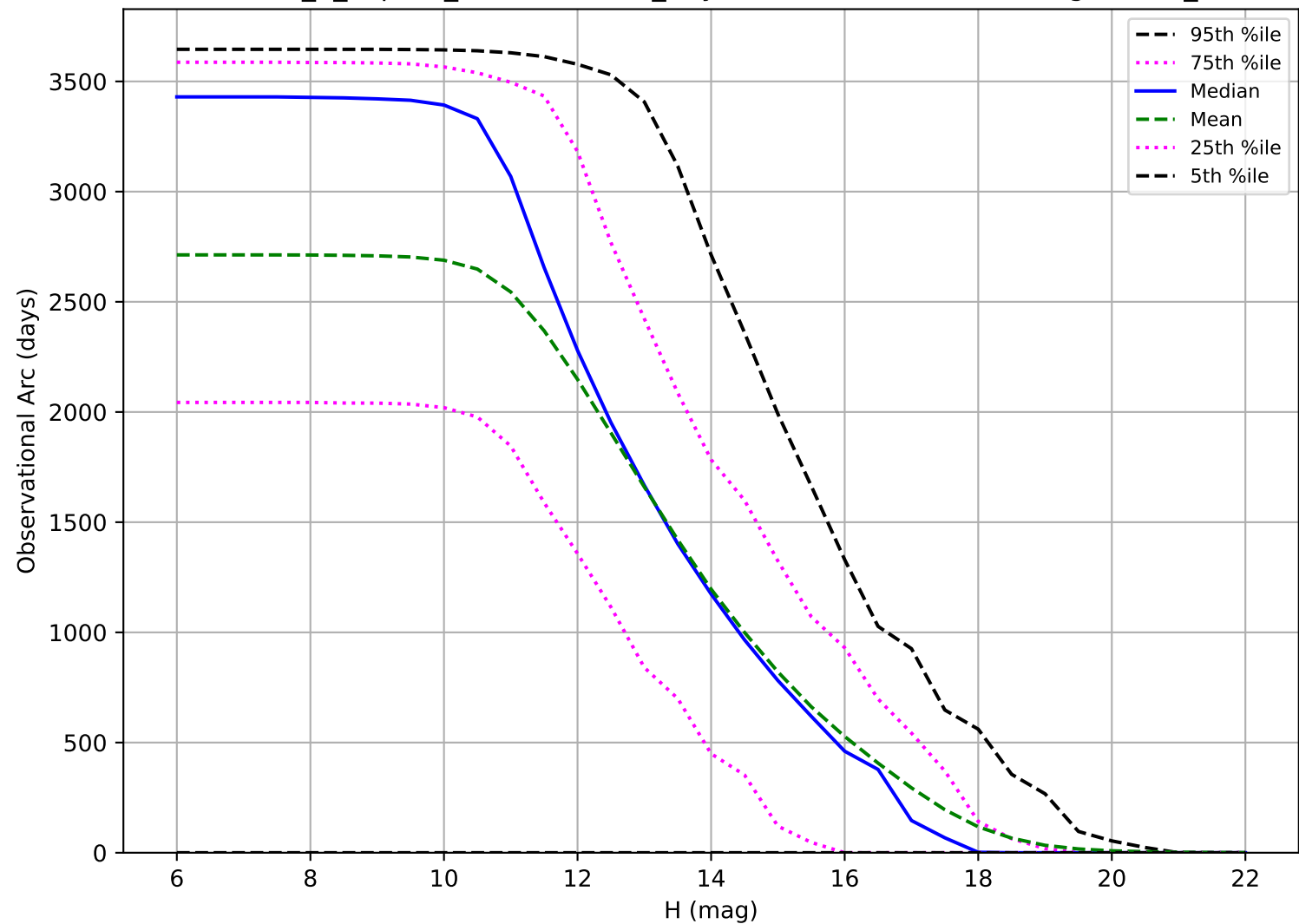
internal_u_expt45_nscale1.2v3.4_10yrs: Observational Arc Length OCC_r5
