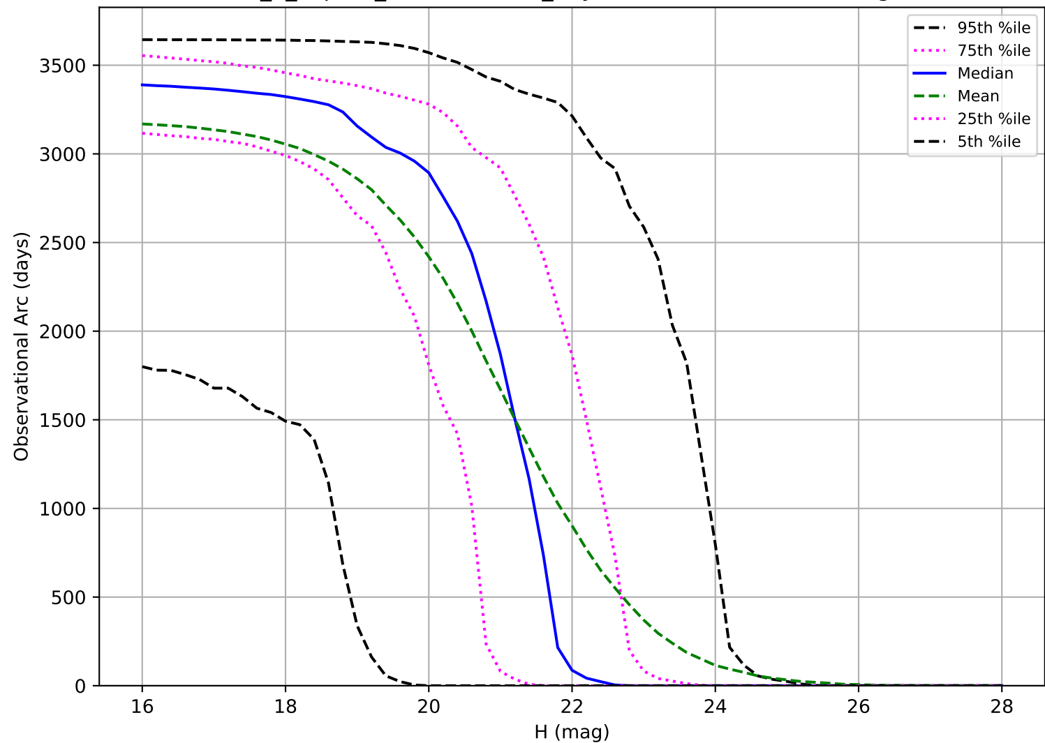
internal_u_expt45_nscale1.2v3.4_10yrs: Observational Arc Length NEO
