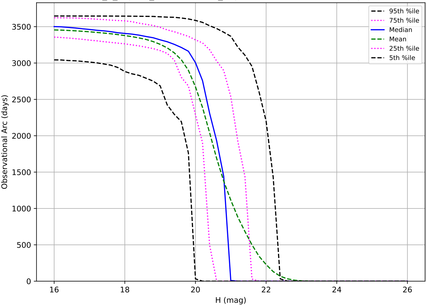
internal_u_expt45_nscale1.2v3.4_10yrs: Observational Arc Length MBA
