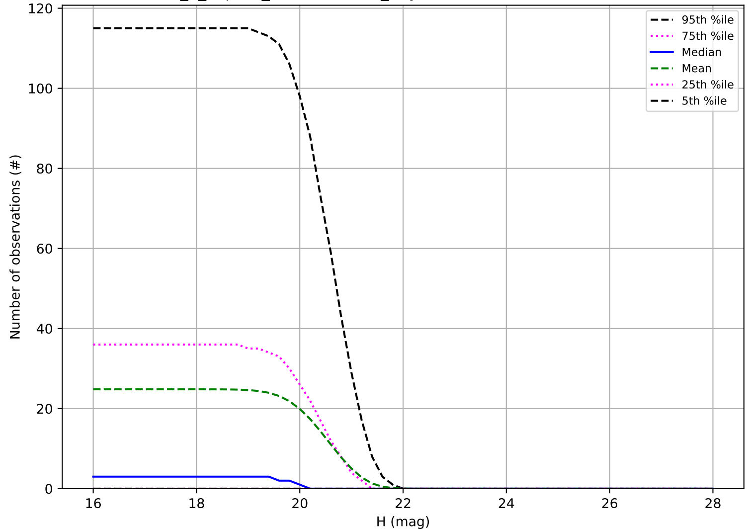
internal_u_expt45_nscale1.2v3.4_10yrs: Number of observations Vatira
