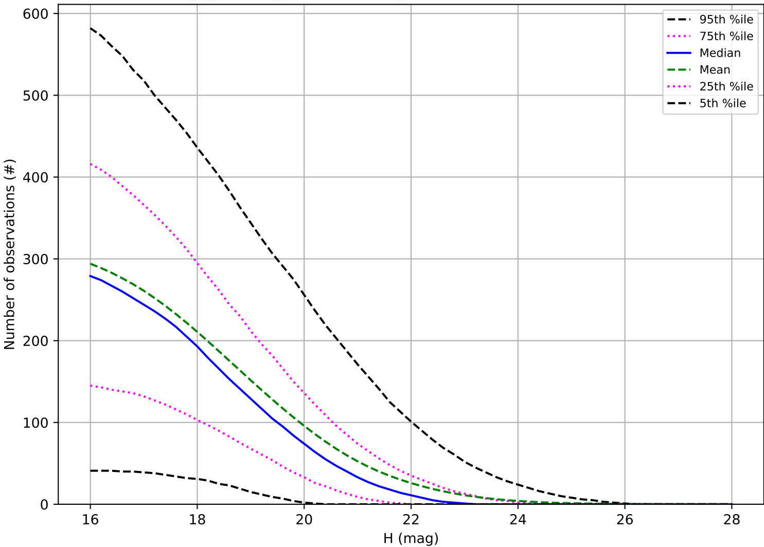
internal_u_expt45_nscale1.2v3.4_10yrs: Number of observations PHA
