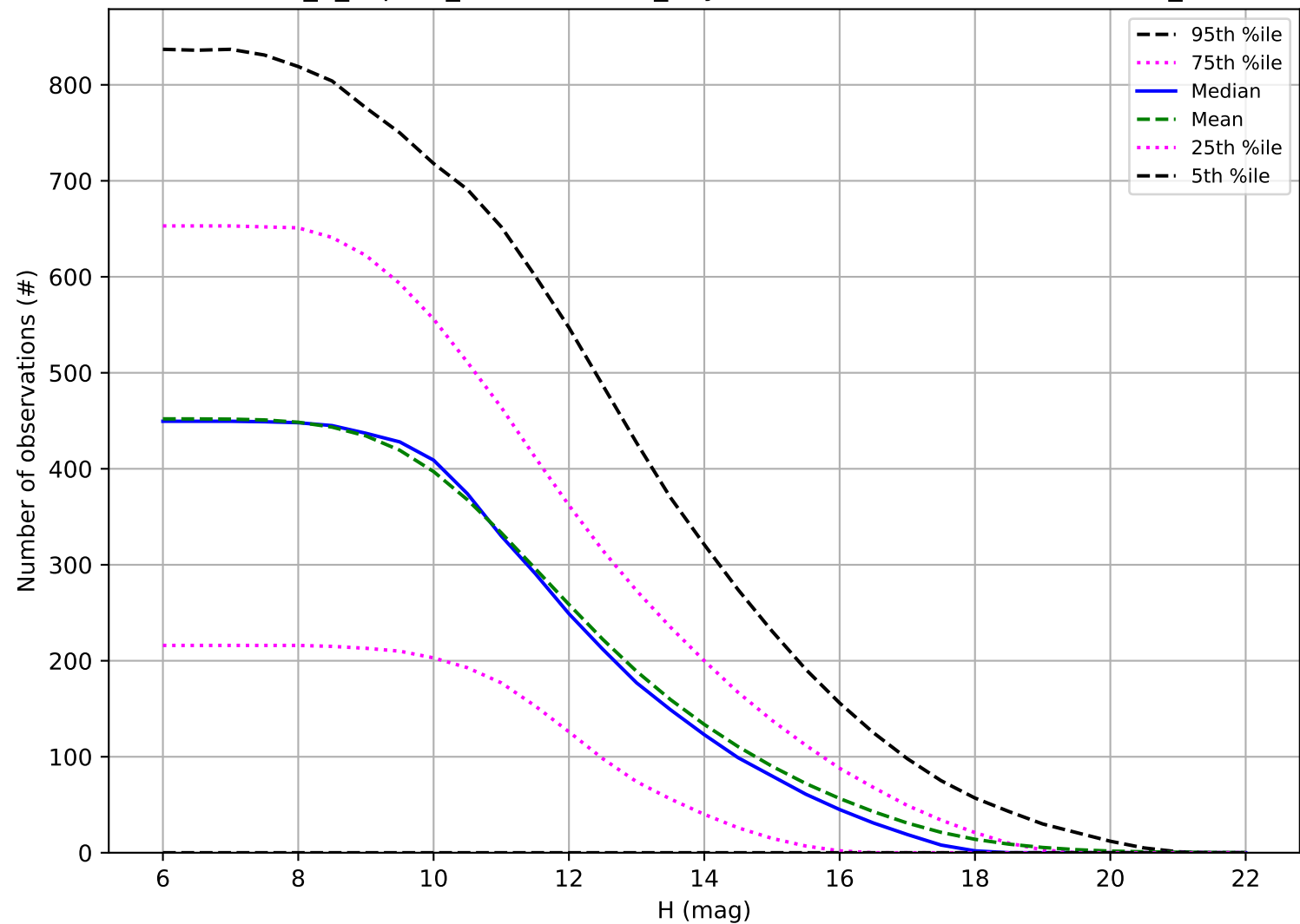
internal_u_expt45_nscale1.2v3.4_10yrs: Number of observations OCC_r5
