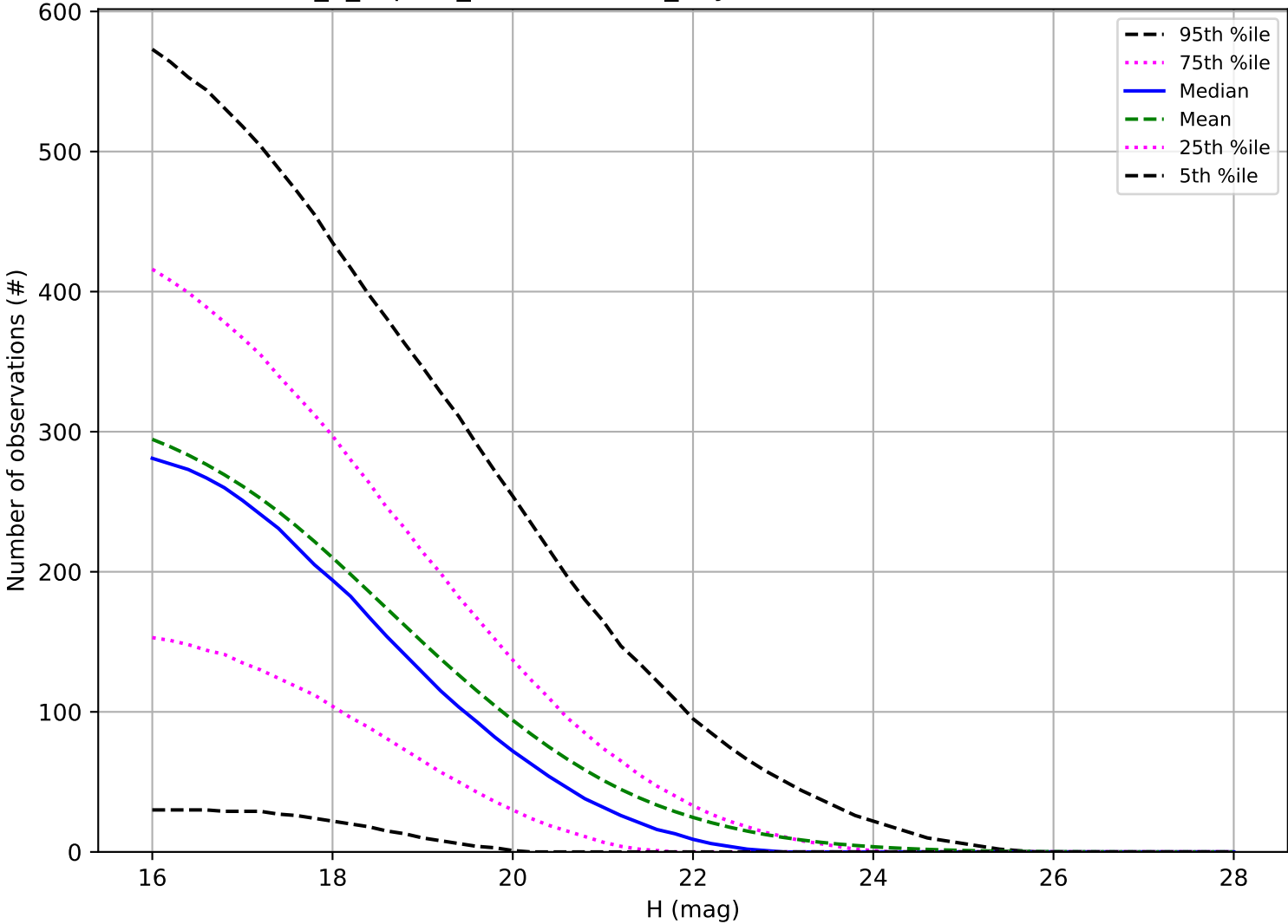
internal_u_expt45_nscale1.2v3.4_10yrs: Number of observations NEO
