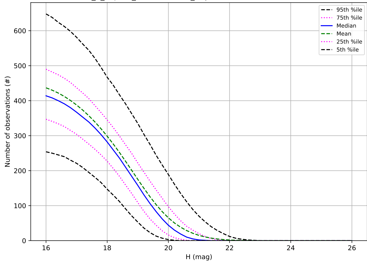
internal_u_expt45_nscale1.2v3.4_10yrs: Number of observations MBA
