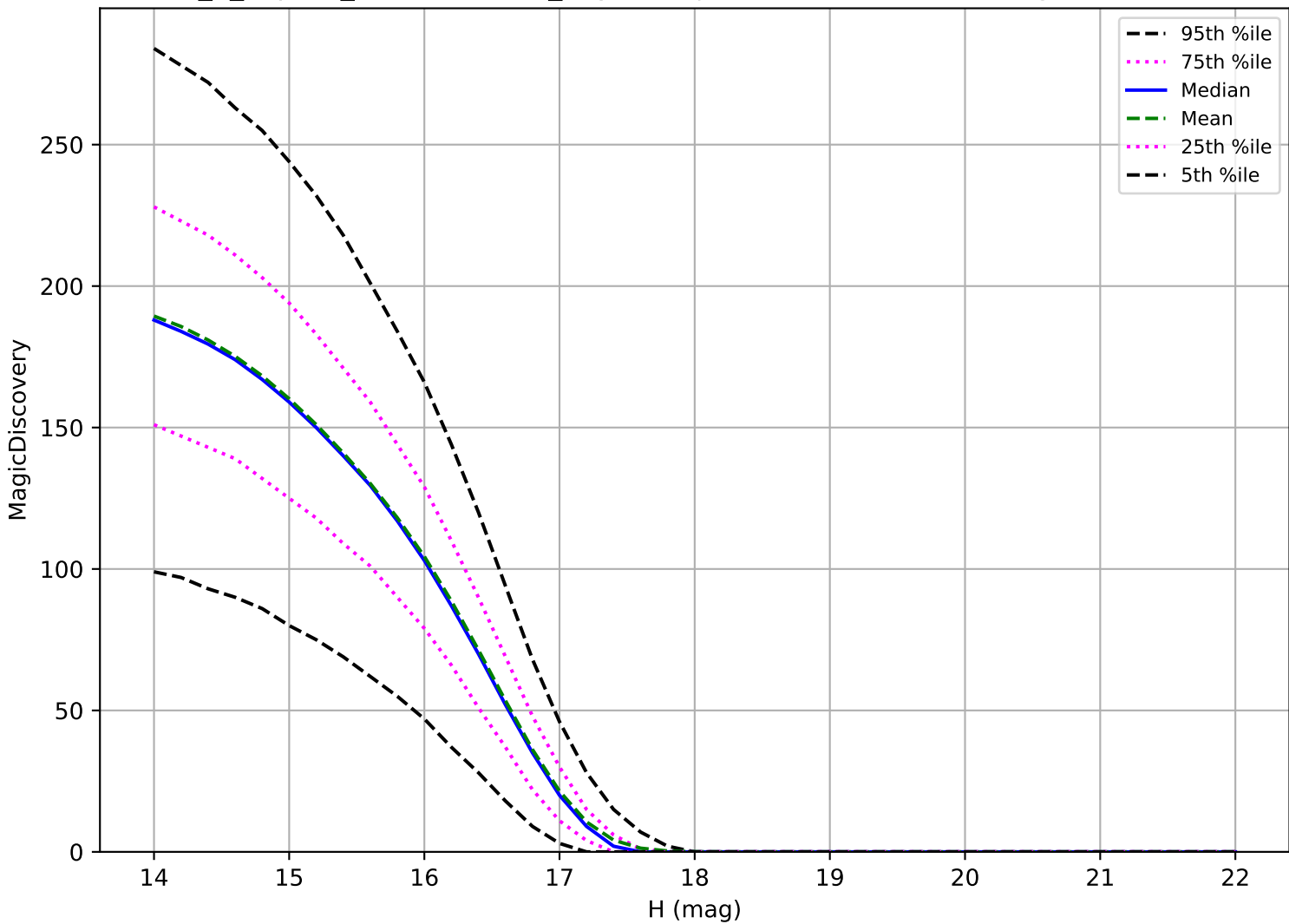
internal_u_expt45_nscale1.2v3.4_10yrs: Trojan 6 detections in 60 nights detection loss
