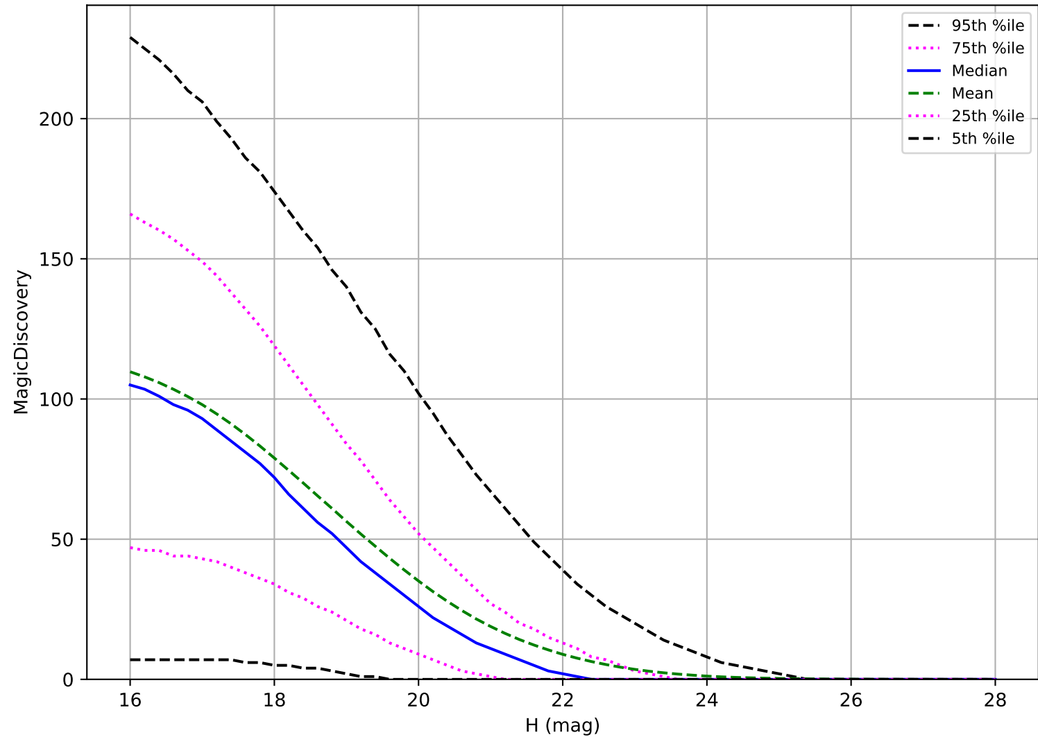
internal_u_expt45_nscale1.2v3.4_10yrs: PHA 6 detections in 60 nights detection loss
