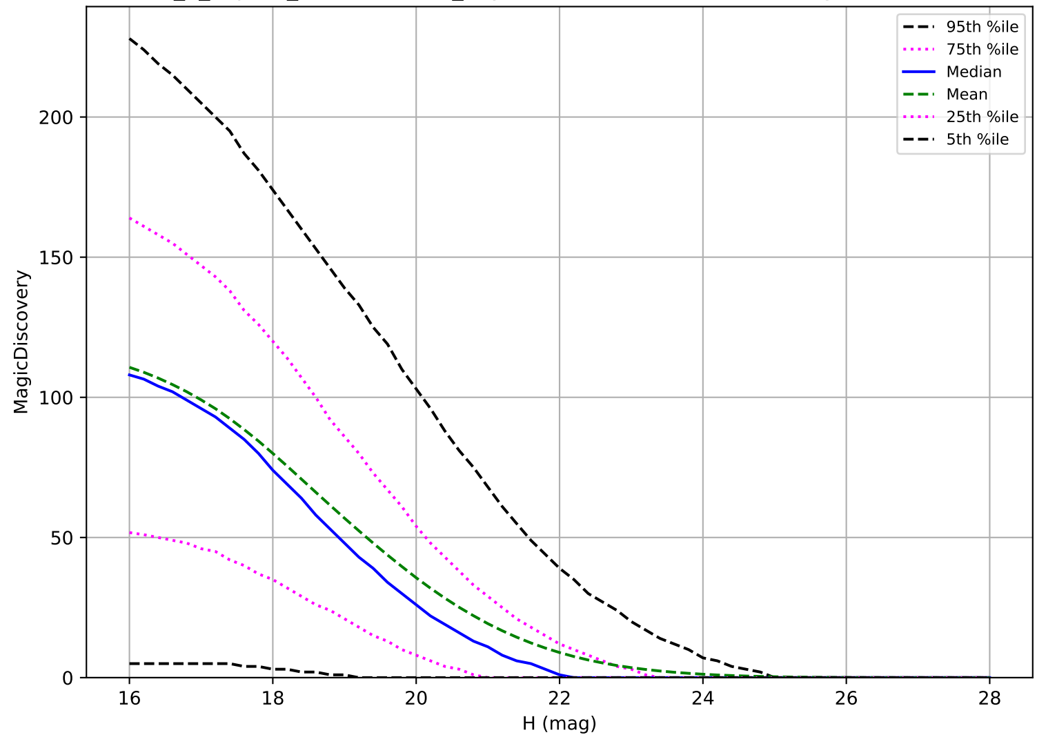
internal_u_expt45_nscale1.2v3.4_10yrs: NEO 6 detections in 60 nights detection loss
