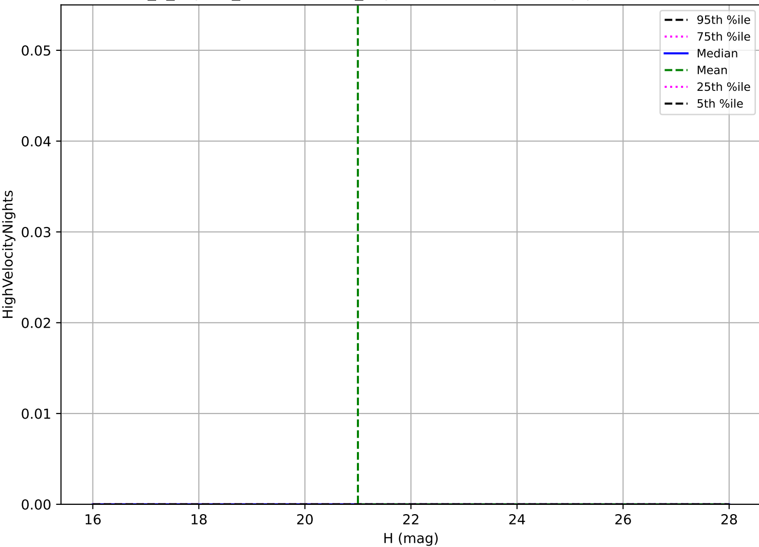
internal_u_expt45_nscale1.2v3.4_10yrs: Vatira High velocity pair detection loss
