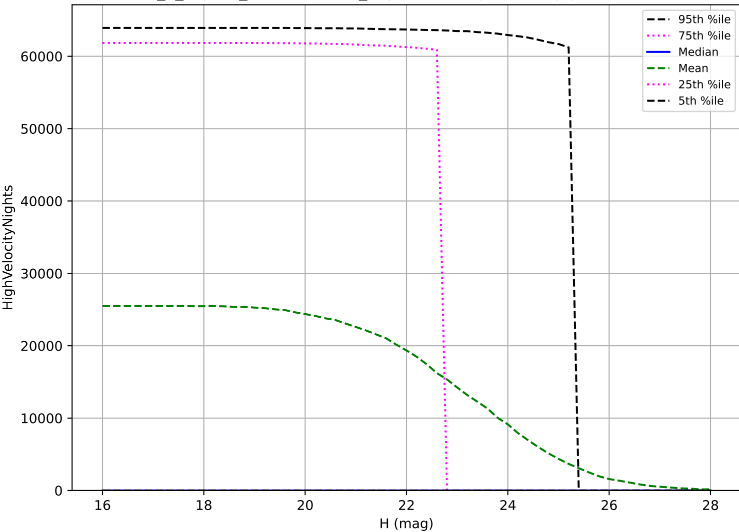
internal_u_expt45_nscale1.2v3.4_10yrs: PHA High velocity pair detection loss
