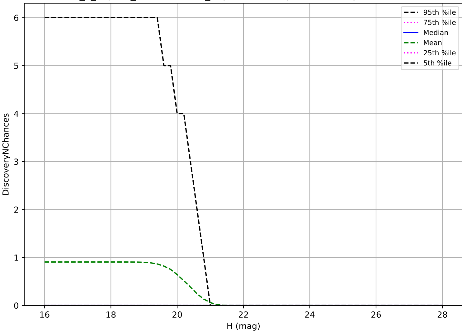
internal_u_expt45_nscale1.2v3.4_10yrs: Vatira 3 pairs in 15 nights detection loss
