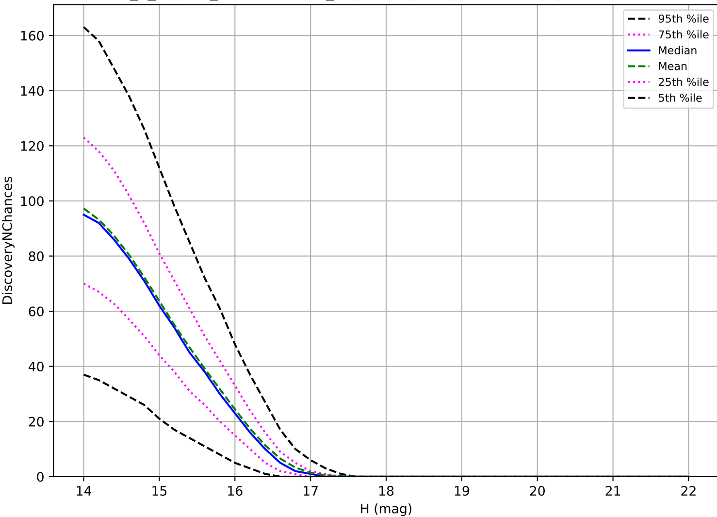
internal_u_expt45_nscale1.2v3.4_10yrs: Trojan 3 pairs in 15 nights detection loss
