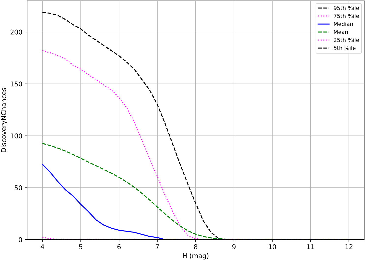
internal_u_expt45_nscale1.2v3.4_10yrs: TNO 3 pairs in 15 nights detection loss
