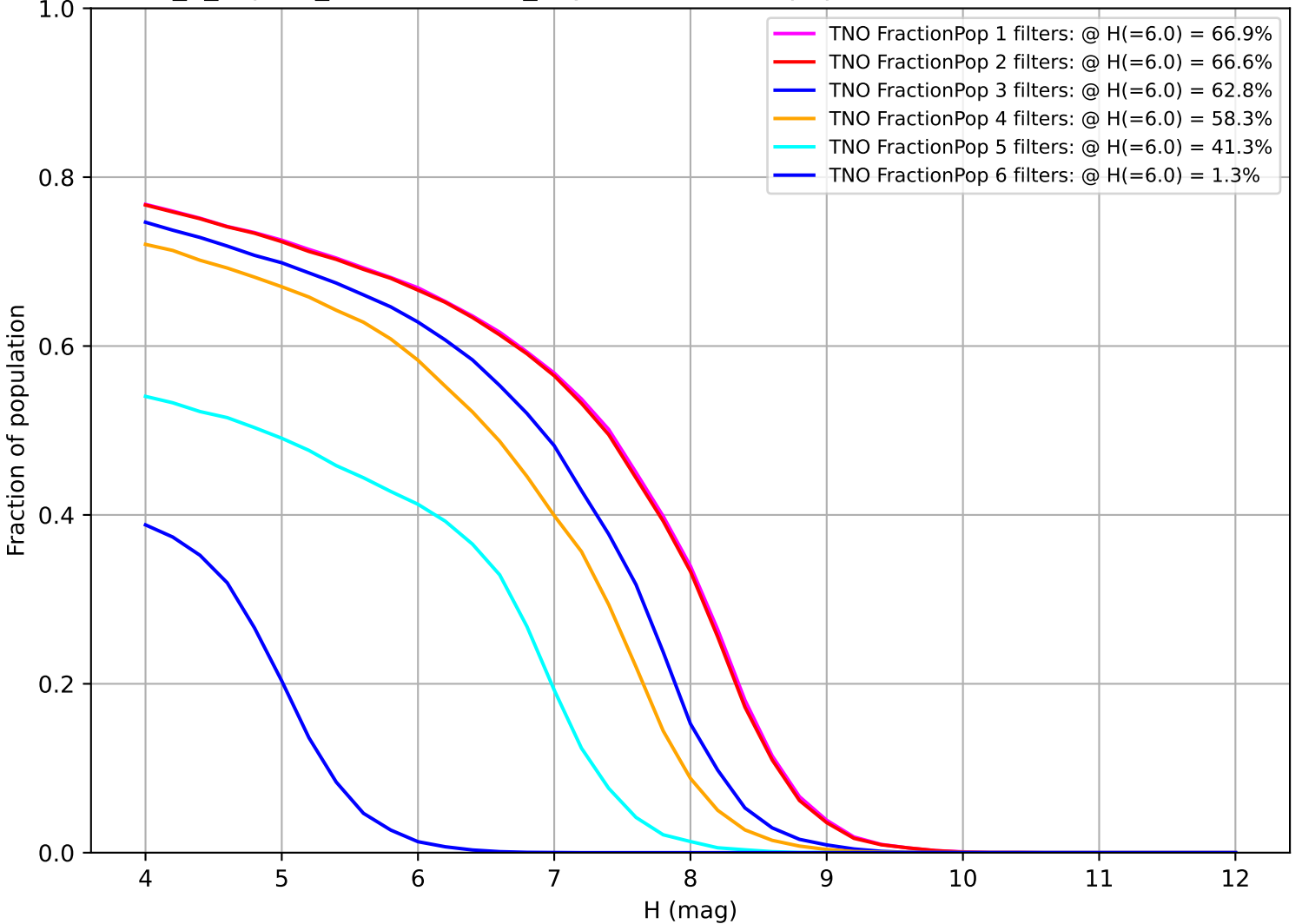
internal_u_expt45_nscale1.2v3.4_10yrs: Fraction of population with colors in X filters TNO
