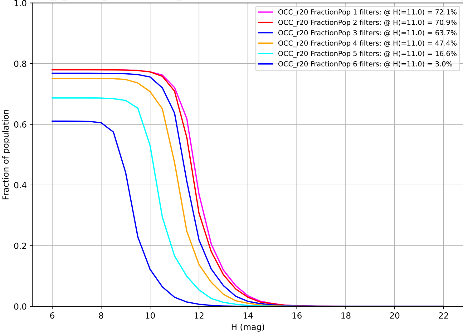
internal_u_expt45_nscale1.2v3.4_10yrs: Fraction of population with colors in X filters OCC_r20
