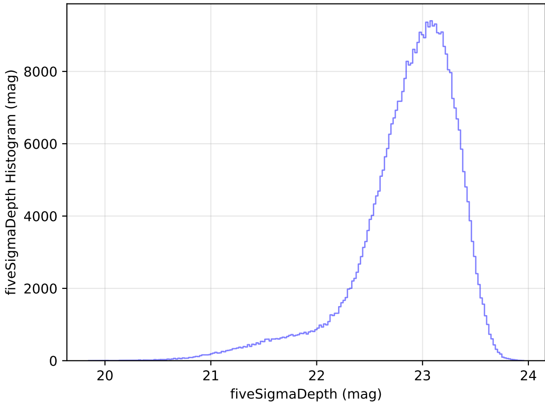
internal_u_expt45_nscale1.2v3.4_10yrs z: fiveSigmaDepth Histogram
